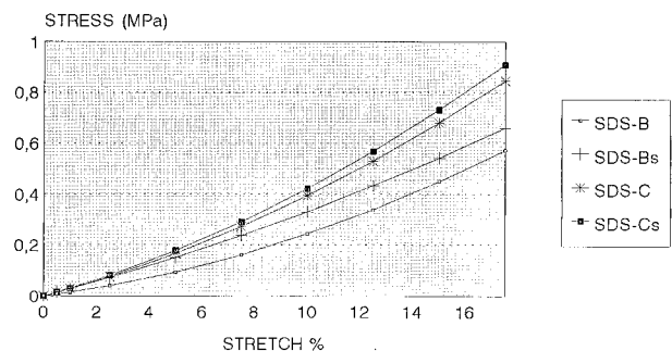
Figure 4 The mean functions for the series treated with SDS. SDS-B: SDS-treated samples obtained from region B. SDS-Bs: sutured (4/0 silk thread) SDS-treated samples from region B. SDS-C: SDS-treated samples obtained from region C. SDS-Cs: sutured (4/0 silk thread) SDS-treated samples from region C. Stress is expressed on the ordinates. Percentage of stretch on the abscissas.
